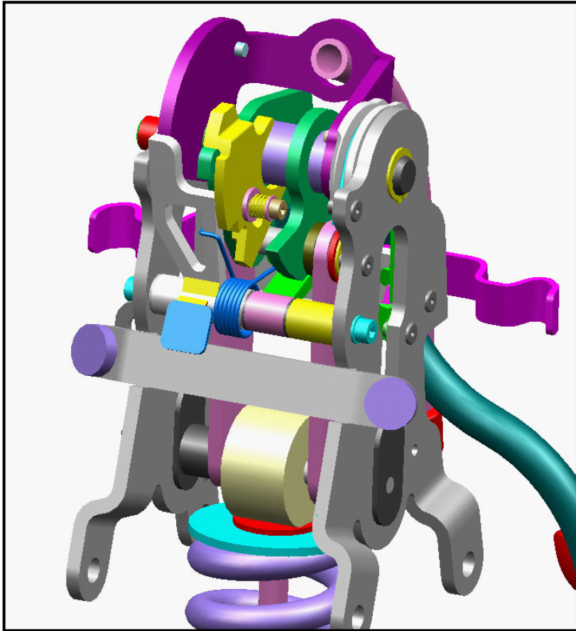
A DETAIL OF THE MAIN STAND LEVER MECHANISM
